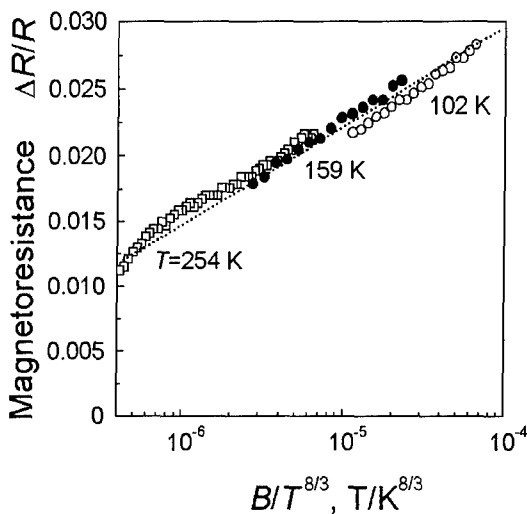
Fig. 4. Parametric dependencies of \text{Fe}_x(\text{SiO}_2)_{1-x} – nano-composite magnetoresistance ( x=0.6 ) in the high field region. The dotted master line is the guide for eye.
