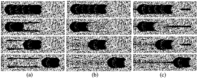
Fig. 6. Images showing the effect of erase power on overwrite. These are images at red wavelength at 50m/s. (a), (b) and (c) are at P_{er} of 11.5mW, 12.75mW and 13.25mW. Top row shows 6T marks and the next three rows are 3T marks written at delays of 0T, 2T and 6T (T-B). Each frame is 2.6μm x 0.8μm.
