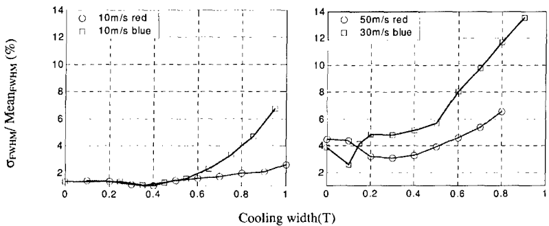
Fig.7. Effect of cooling width on overwrite jitter
