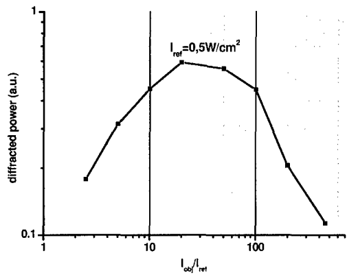
Figure 3. Diffracted power as a function of the intensity ratio of object and reference beams with beam radius of 0.11 mm.
