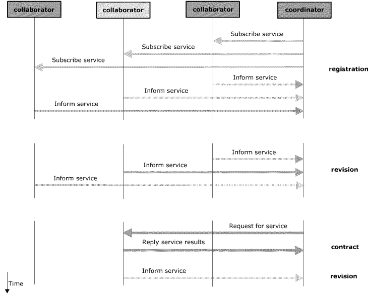
Figure 4 – Contraction based on Acquaintance Model exploitation
