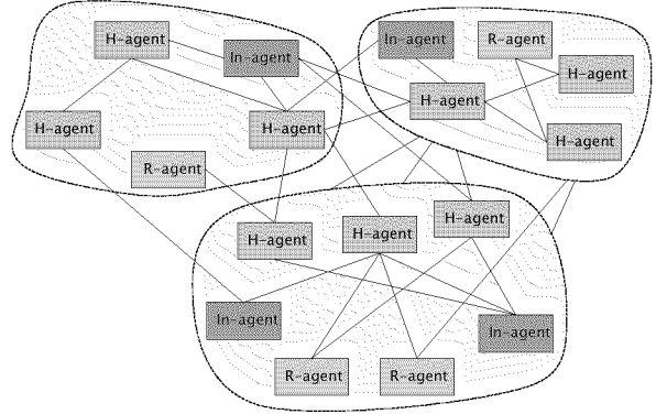
Figure 1 – CPlanT Multi-Agent Architecture
