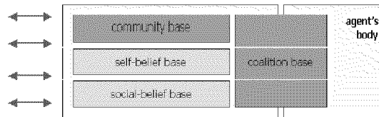
Figure 2 – Structure of the CPlanT Acquaintance Model
