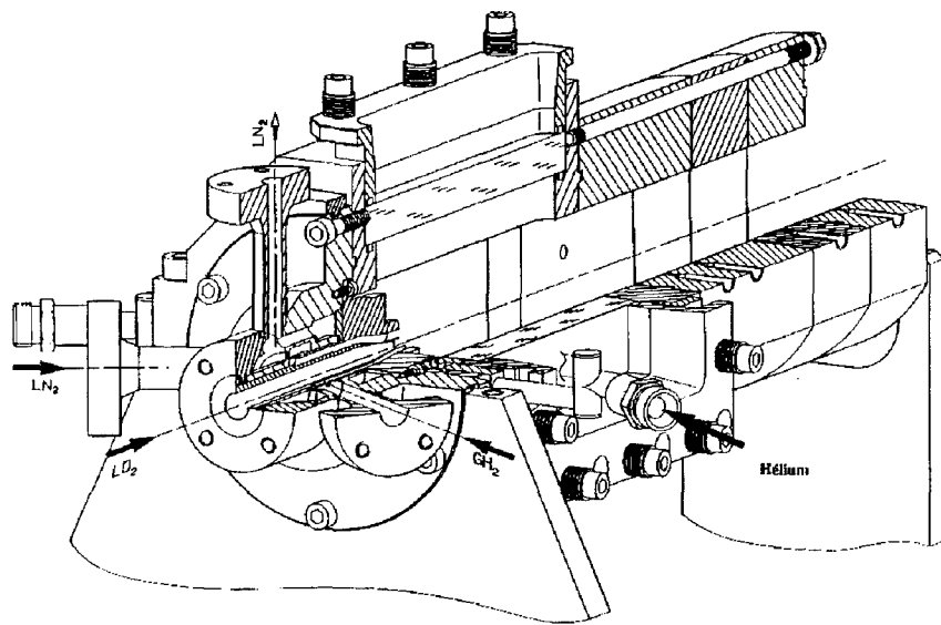
Figure 1: MASCOTTE Combustor
