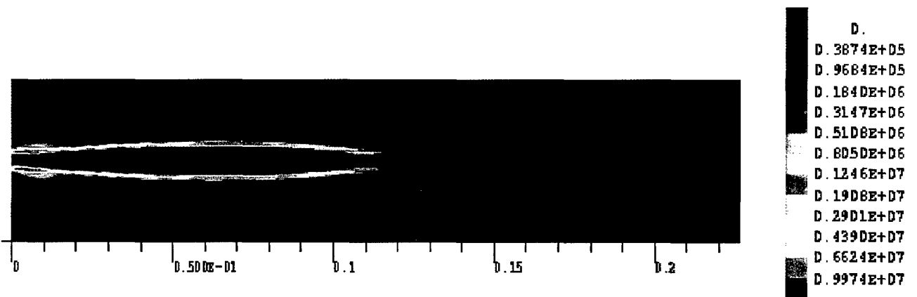
Figure 14 : Reactive rate (mol/kg/s) : Liquid, q - \omega , oxygen (injection except \sigma )
