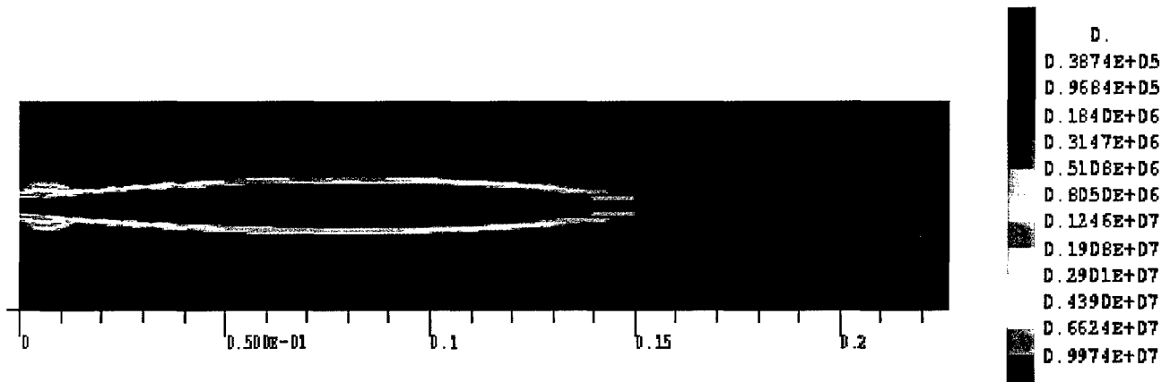
Figure 13 : Reactive rate (mol/kg/s) : CFM, k - \epsilon , Gas – Liquid (~1:1)
