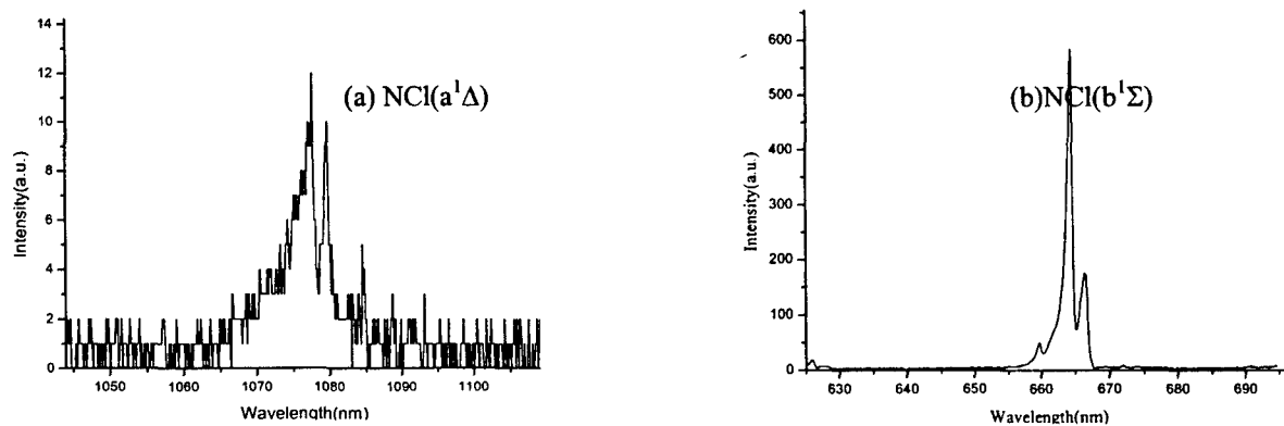
Figure 2 Spectra of NCl( a^1\Delta ) and NCl( b^1\Sigma ) emission
