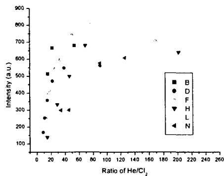
Figure 4 The intensity of NCl( b^1\Sigma ) emission dependent on the ratios of He and \text{Cl}_2 ,
