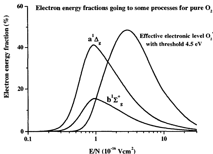
Fig.9. Electron energy fraction going to some processes for pure O 2
