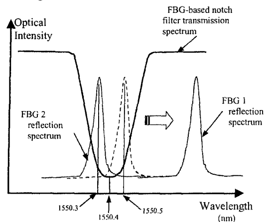
FIGURE 3: Optical intensity spectra for FBG's and FBG-based notch filter when FBG 1 is strained.
