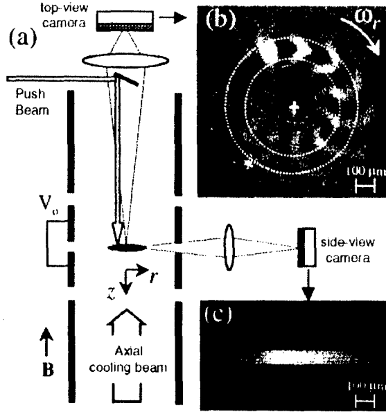
FIGURE 1. (a) Schematic of the cylindrical Penning-Malmberg trap and imaging diagnostics. (b) Top-view image of the differential fluorescence \Delta I(r, \theta) for an \alpha = 0.042 \text{Be}^+ ion crystal. The annular region defined by the dotted circles is analyzed to obtain dispersion relationship data. (c) Side view image of an \alpha = 0.042 crystal.
