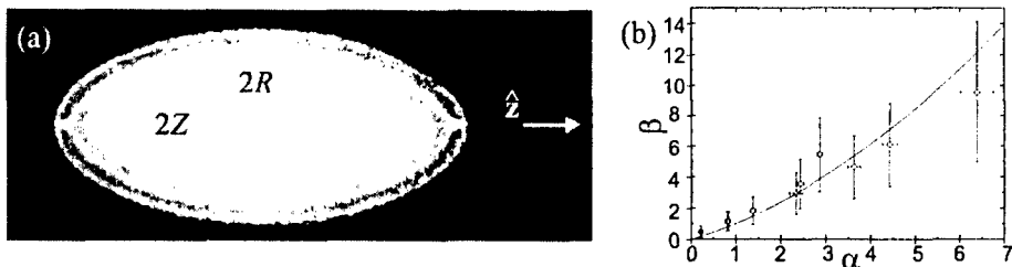
FIGURE 3. (a) Example of a Coulomb crystal with a shape and density described well by cold fluid theory with \omega_p = 0 . The ions are arranged in closed spheroidal shells. (b) The relation between \alpha and \beta as given by cold fluid theory (line). \beta for a string-of-discs state crystal (o) calculated from experimental parameters using Eq. (3) with \omega_p = 0.31 \times \omega_{rf} .
