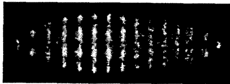
FIGURE 5. String-of-discs structure showing radial ordering. The image was obtained by averaging over 5 frames ( \approx 1 s).
