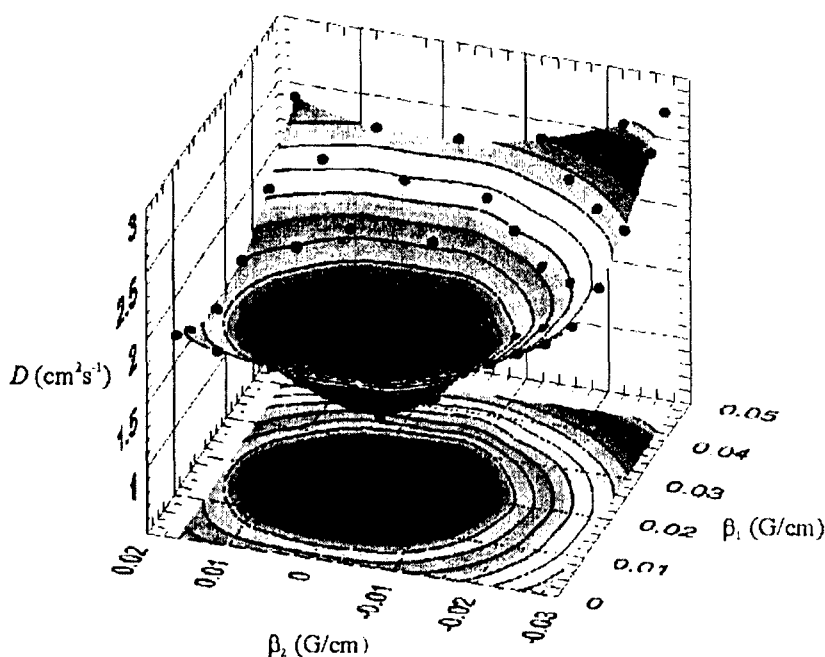
FIGURE 5. Diffusion from the application of a quadrupole field. This data is taken at B_z = 100 \text{ G} , r_0 = 0.95 \text{ cm} , and \omega = 2.0 \times 10^6 \text{ rad s}^{-1} . We choose values of \beta_1 and \beta_2 in a checkerboard pattern and the data (solid dots) show that there is an optimal quadrupole field and that diffusion increases away from this optimal value.
