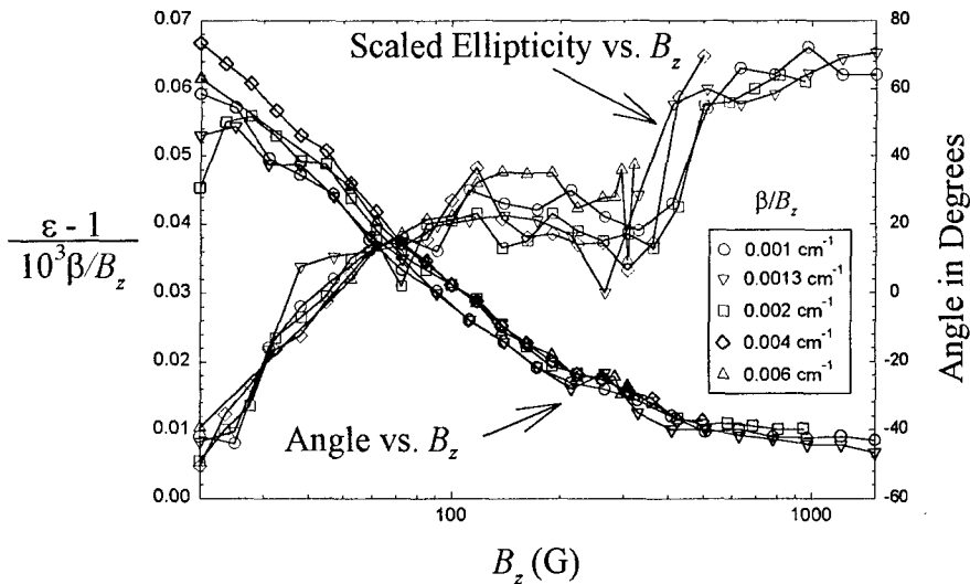
FIGURE 2. Varying B_z changes \omega and thus \overline{\omega t_b} . \epsilon(B_z) - 1 approaches zero at low B_z (large \omega t_b ) and is proportional to \beta . \theta_p \approx \theta_n = -45^\circ at large B_z and the change in \theta_p(B_z) is likely due to imaging fields.
