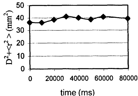
FIGURE 4. Comparison of asymmetry-dominated diocotron decay (left) with a decay dominated by rotational pumping (right). The new regime is characterized by non-conservation of angular momentum (Figure 4d, see text).
