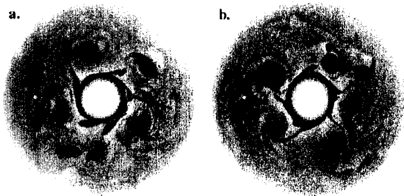
FIGURE 6. The long-term evolution of a continuously injected plasma column. The circumference of the original column is continuously supplied with electrons from the photocathode. Figure a) shows the early stages of filamentation (A) perturbation and (B) extension. Figure b) shows the later stages (C) capture and (D) spiraling. Images are representative of development at 200ms.
