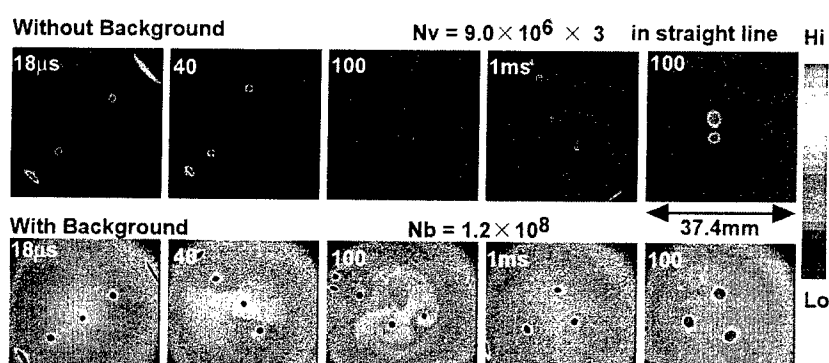
FIGURE 9. Three clumps in straight line are crystallized in the presence of a low-level background vorticity distribution.
