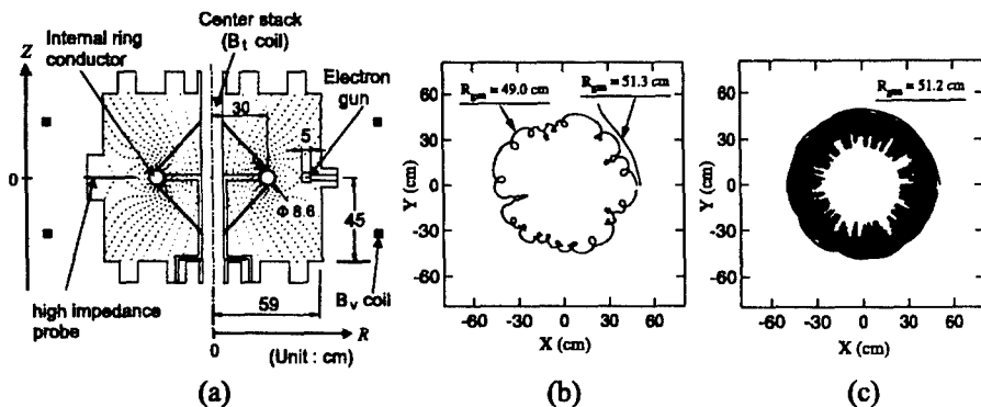
FIGURE 1. (a) Schematic view of the Proto-RT device. (b) Typical orbits of electrons emitted from inside ( R_{gun} = 49.0 cm) and outside ( R_{gun} = 51.3 cm) the trapping region (c) A typical orbit (toroidal projection) of electrons emitted from near an X-point ( R_{gun} = 51.2 cm)
