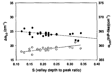
Figure 3.. \Delta\omega_{LO}(\omega_{LO1}-\omega_{LO2}) (● ) and \omega_{LO2} (InP-like) (○) vs S
