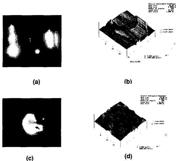
Figure 2. The field emission patterns of the DLC films and AFM images of the emitted spots: (a) DLC at 16\text{ V}/\mu\text{m} , (b) an emitted spot of (a), (c) DLC 20\text{ V}/\mu\text{m} and (d) an emitted spot of (c).
