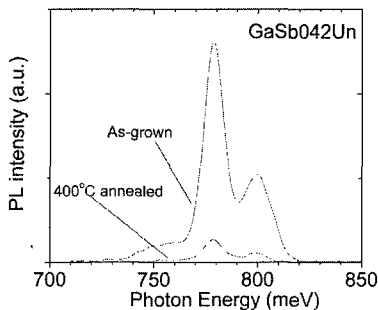
Figure 3 PL spectra of the as-grown and 400°C annealed GaSb042Un undoped GaSb samples. The measurements were performed at T=10\text{K} .
