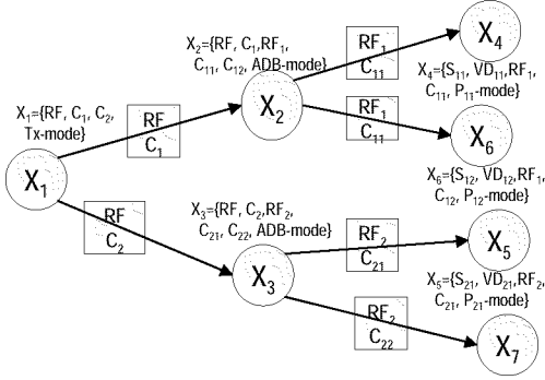
Figure 2: Decomposition graph of extended IFE system description. Here an oval corresponds to a vertex, and a block corresponds to a sepsset. We specify the variables associated with each vertex in the graph.
