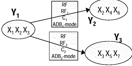
Figure 3: Clan graph of extended IFE system description.
