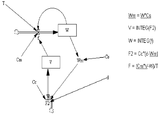
Figure 3. Forrester diagram
