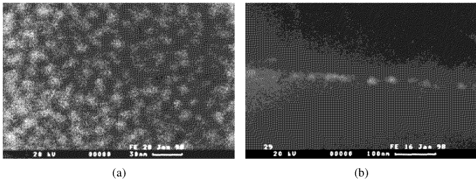
Fig. 1. SEM image of fabricated monolayer. (a) plain view and (b) cross view.
