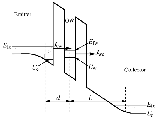
Fig. 1. The energy diagram of the DBRTS in the regime of the resonant tunneling.
