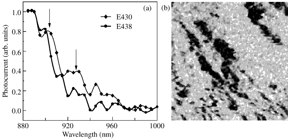
Fig. 2. (a) STM spectra of photoconductivity for structures with InAs/GaAs quantum dots located near sample surface. The thickness of the overgrown layer for sample E438 is 2 nm, for sample E430—1.5 nm. (b) Photoresponse distribution across the surface of a sample containing a quantum well at a 250 nm depth. Frame size is 1 \times 1 \mu\text{m} .
