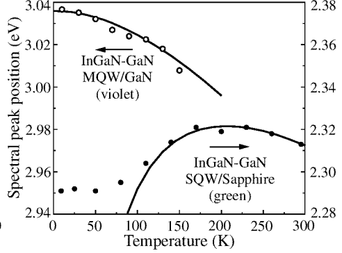
Fig. 3. PL spectral peak position of two InGaN samples: 1) open circles are for homoepitaxial MQW structure (grown by MOCVD on bulk GaN substrate obtained by sublimation method); pumping wavelength is 325 nm [18]; 2) solid circles are for green LED SQW structure on sapphire substrate; pumping wavelength is 442 nm [13].
