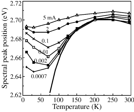
Fig. 2. EL spectral peak position of blue InGaN SQW LED at different current [13]. Thick curve is calculated according to Eq. (2). Fitting parameter s is 31.5 meV.
