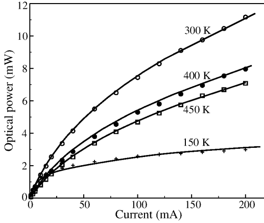
Fig. 1. Light-current characteristics of green Nichia InGaN SQW LED in temperature range up to 450 K. Curves are calculated with recombination coefficients as fitting parameters. Diode area is 7 \times 10^{-4} \text{ cm}^2 .
