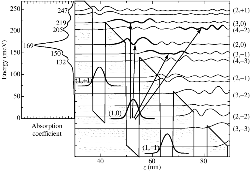
Fig. 2. Conduction profile, energy levels and electron distributions for four superlattice periods with an electric field of 60 kV/cm. The experimental observed transitions are indicated by arrows. The calculated absorption coefficient is shown on the left.
