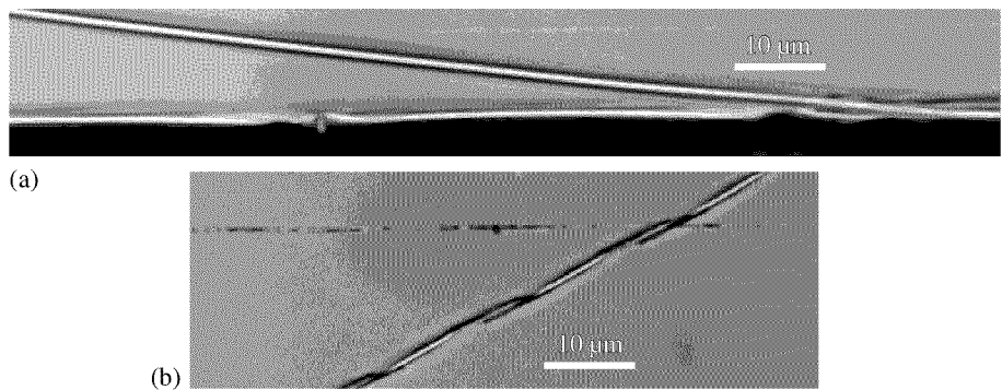
Fig. 2. Photographs of a tube (a) and a helical coil (b) of 1.5\text{ }\mu\text{m} in diameter made from a \text{Ge}_{0.4}\text{Si}_{0.6}/\text{Si} bilayer. Thicknesses of \text{Ge}_{0.4}\text{Si}_{0.6} and Si films were 10 and 20 nm, respectively.
