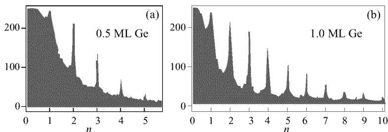
Fig. 2. Line scans in [001] growth direction of zero beam spot in diffraction patterns from multilayer structures A (a) and B (b). In the case of sample B the number of satellites n is twice as large as in sample A.
