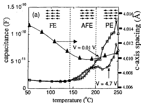
Figure 3- Structural transition (inflection in c-axis lattice spacing) and dielectric anomaly as function of temperature.
