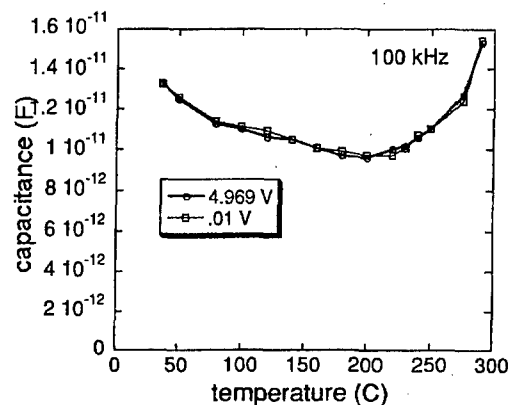
Figure 4. Capacitance vs. temperature for an alloy \text{K}(\text{Ta}_{0.5}\text{Nb}_{0.5})\text{O}_3 film
