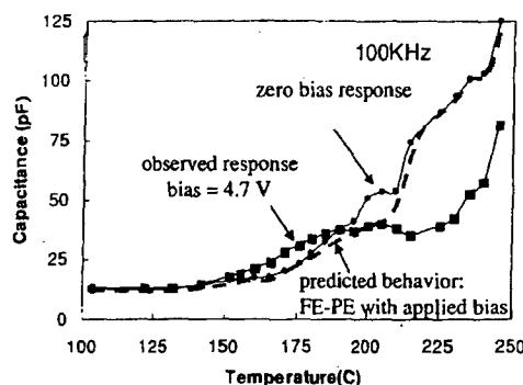
Figure 1 Capacitance for inter-digitated capacitor on 1x1 \text{KTaO}_3/\text{KNbO}_3 superlattice at 0 and 4.7 V dc bias. Also shown is the expected behavior for a ferroelectric (FE)-paraelectric (PE) system based on qualitative prediction only.
