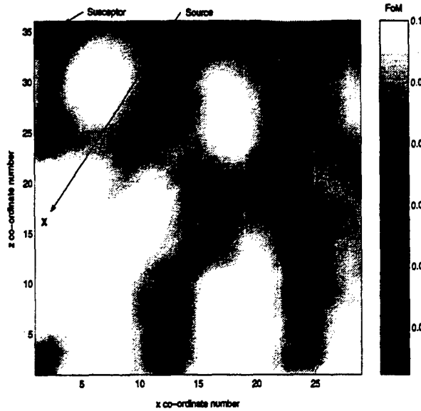
Figure 4: False colour plot of final field distribution on surface of dielectric slab after non-lossy simulation. The x and z axes are marked in FDTD cells. Source and susceptor positions are indicated on the figure.
