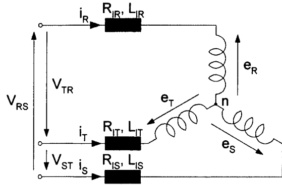
Figure 1. The windings are star connected.
