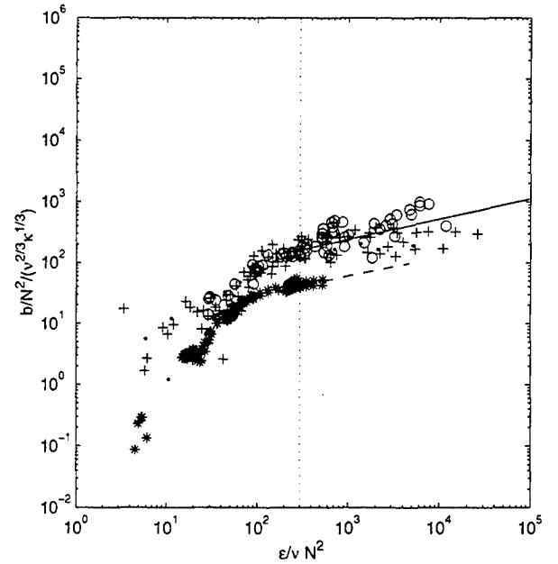
Figure 4. (b/N^2)/(\nu^{2/3}\kappa^{1/3}) vs \epsilon/\nu N^2 ; \cdot , Stillinger et al. (1983b); \circ , Rohr (1985); + , Itsweire et al. (1987); * , Ivey et al. (1998). The equations of the lines are given in the text.
