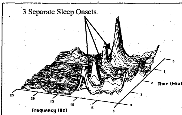
Figure 3C: 31 Hrs Awake
