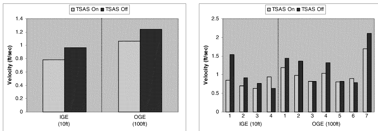
Figure 4. Simulator Velocity Errors – Hover Displays On
