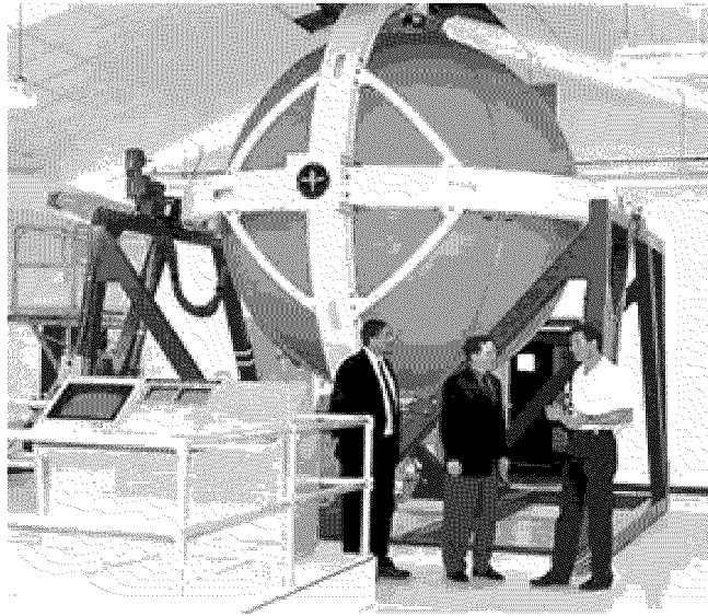
Figure 6. Visual Vestibular Sphere Device (VVSD)
