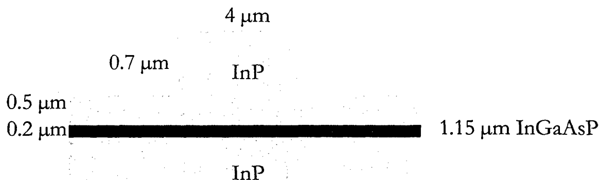
Figure 7 : Example of optical InP passive waveguide for switching matrixes.
