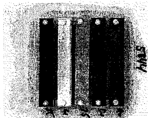
Figure 2. Typical Corrosion Test Card Containing 5 Metallic Coupons; 4 Cards Per Test Site
