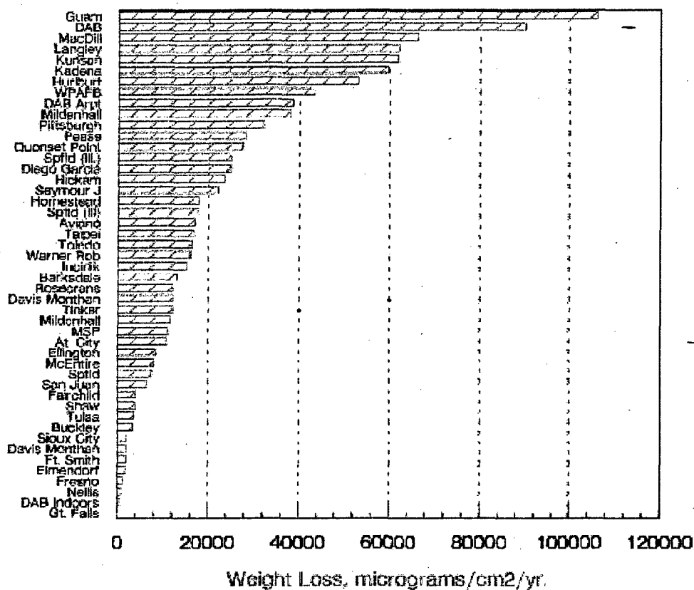
FIGURE 7. WEIGHT LOSS OF 1010 STEEL IN OUTDOOR BASE ENVIRONMENTS
