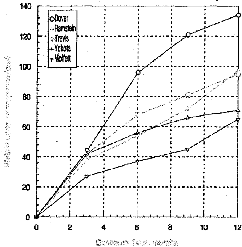
FIGURE 4. CORROSION OF 6061 ALUMINUM DURING OUTDOOR EXPOSURES
