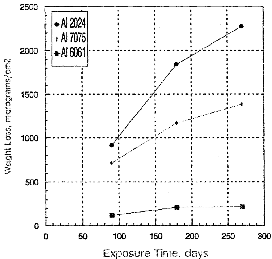
FIGURE 6. EFFECTS OF ALLOY TYPE ON CORROSION OF ALUMINUM
