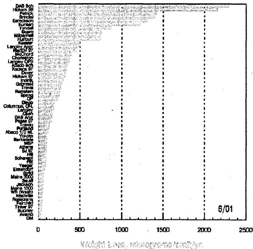
FIGURE 5. WEIGHT LOSS OF 7075 ALUMINUM AT OUTDOOR FIELD SITES
