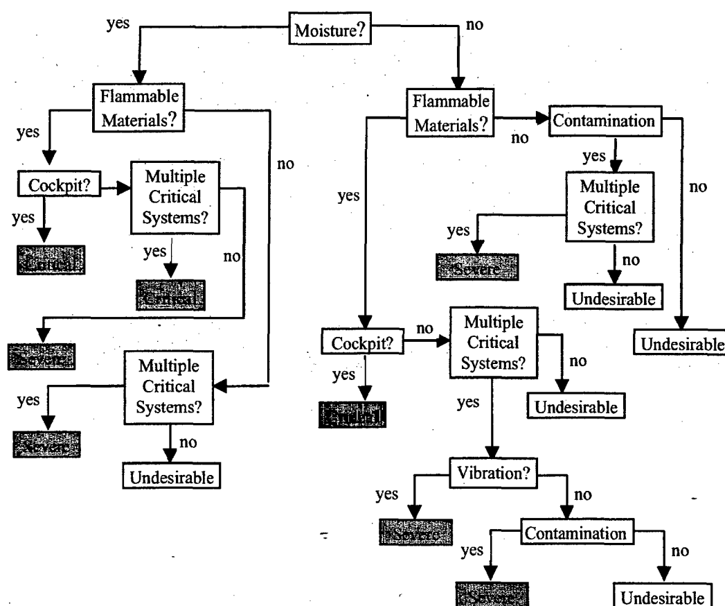
Figure 3: Example Fault graph for Wire Cracking
