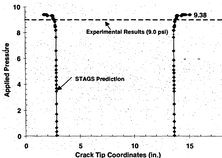
Figure 7. Measured and predicted residual strength
