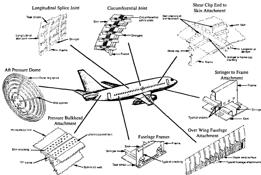
Figure 1. Susceptible widespread fatigue damage locations
