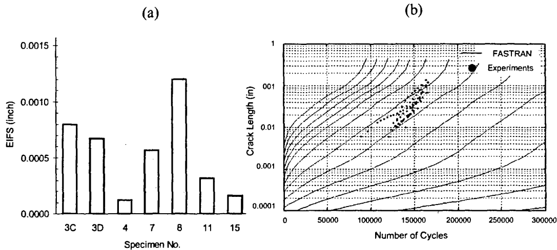
Figure 4. (a) EIFS distribution and (b) correlation between experiments and analysis using FASTRAN with different values of EIFS.
