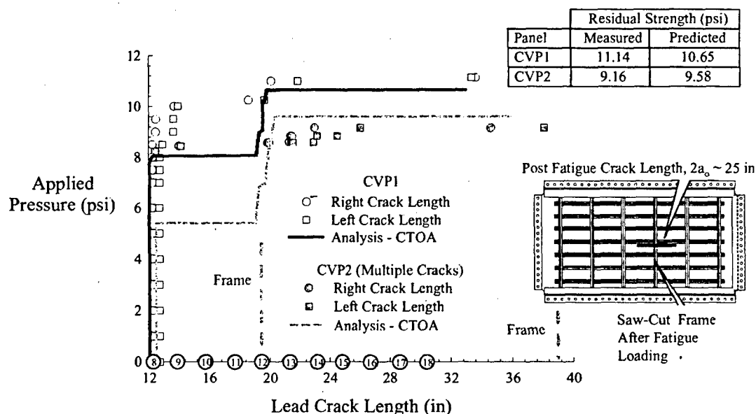
Figure 6. Measured and predicted residual strength
