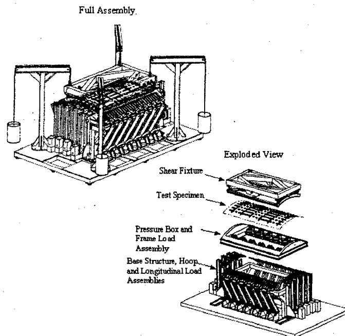
Figure 5. Full-Scale Aircraft Structural Test Evaluation and Research fixture
