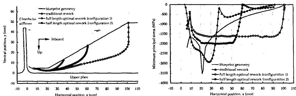
Figure 2: Comparison of blueprint, traditional and optimised rework shapes (shown inverted) and elastic boundary stress distributions at CPLT loading of +7.33g for SRO#2.
