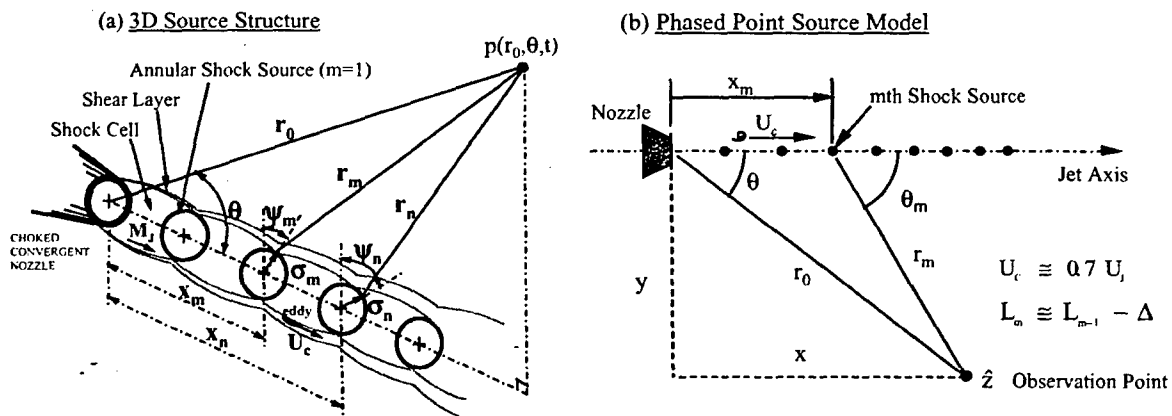
Fig.10 Shock Noise Source Model
