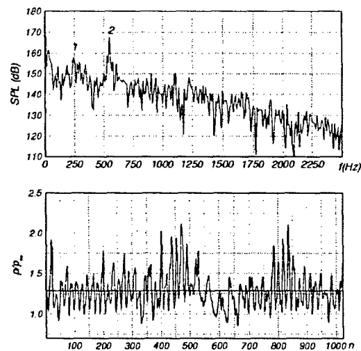
Figure 10 Unsteady pressure fluctuations and frequency spectra of the cavity with ramp.
