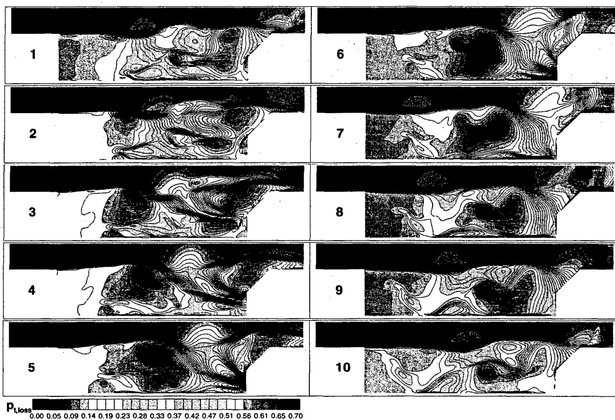
Figure 11 Instantaneous total pressure loss contours produced by the Euler with boundary layer model.
