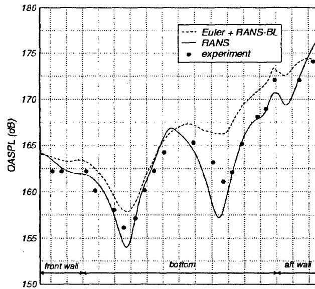
Figure 9 Overall sound pressure level (OASPL) along the centreline of the simple rectangular cavity (the experimental values are obtained from the data presented in Ref. [7]).
