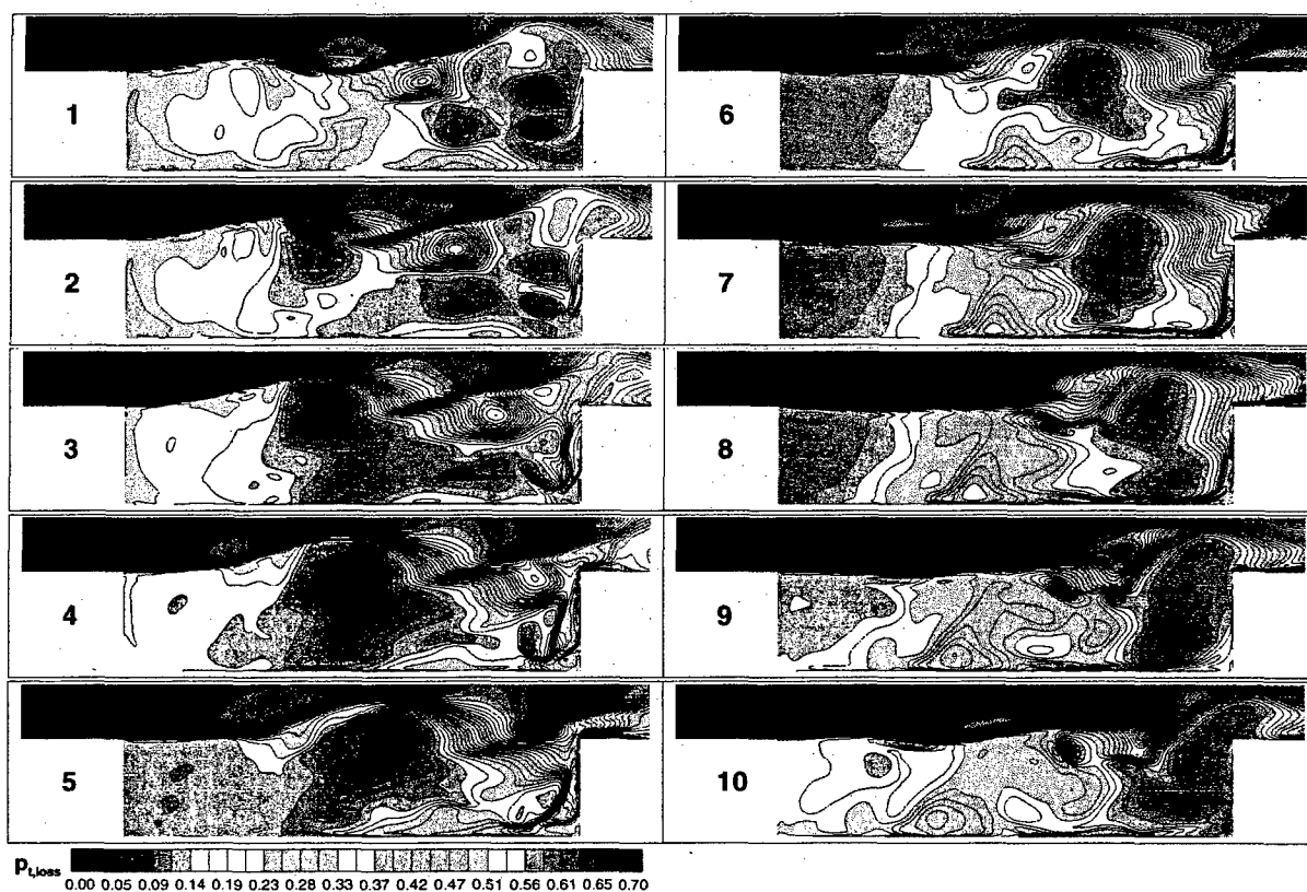
Figure 7 Instantaneous total pressure loss contours produced by the Euler with boundary layer model.
