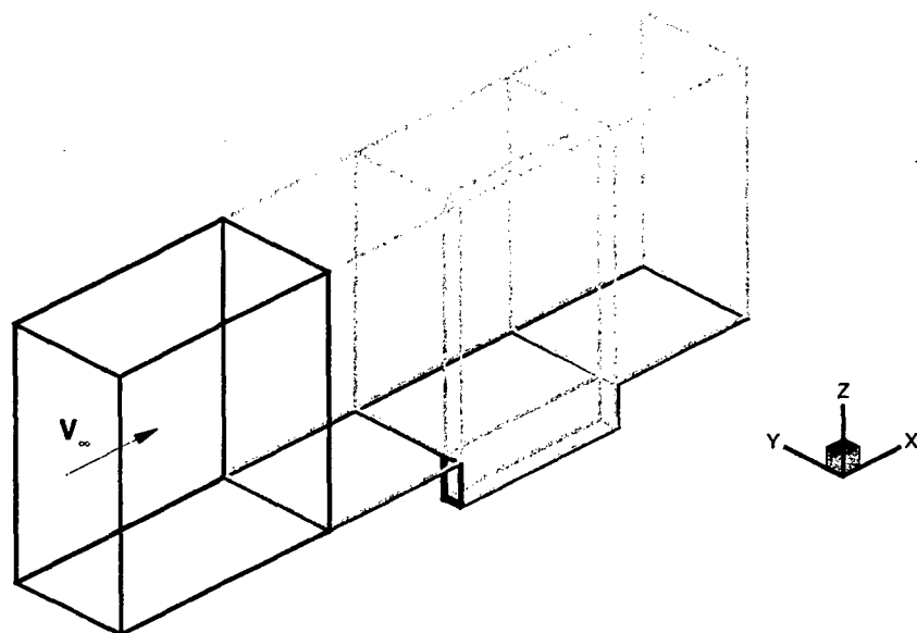
Figure 1 Flow domain modelling of the cavity flowfield.
