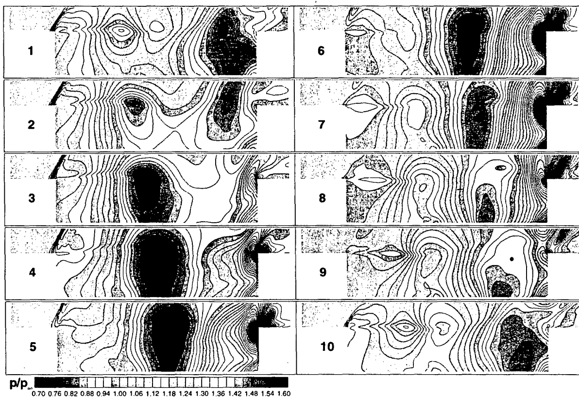
Figure 6 Instantaneous static pressure contours produced by the RANS model.
