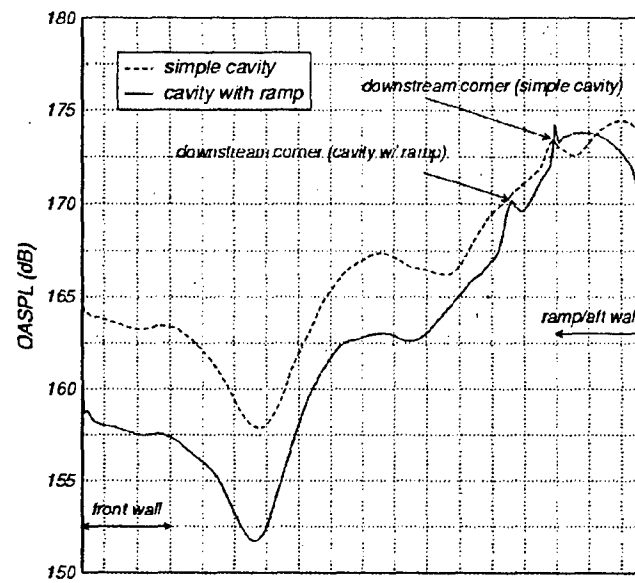
Figure 13 Effect of the trailing edge geometries to the overall sound pressure level.
