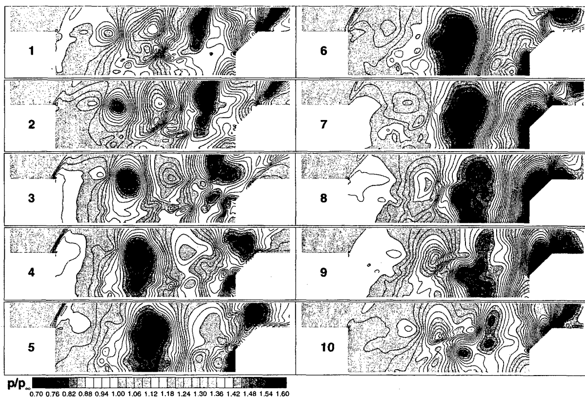
Figure 12 Instantaneous static pressure contours produced by the Euler with boundary layer model.
