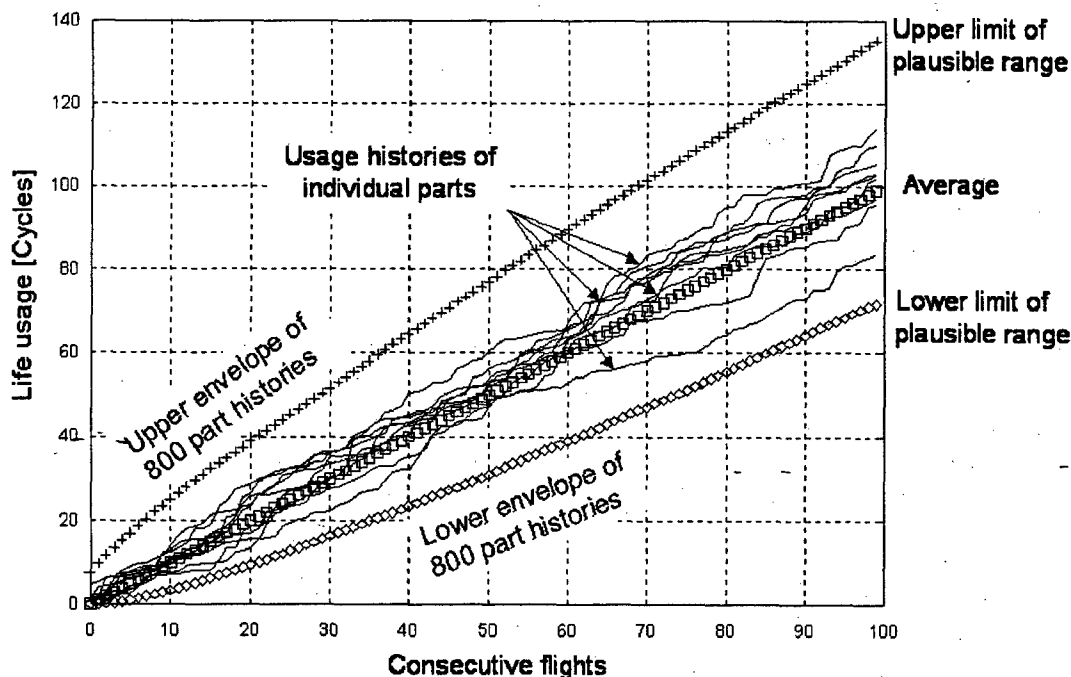
Figure 6: Scatter in accumulated life usage
