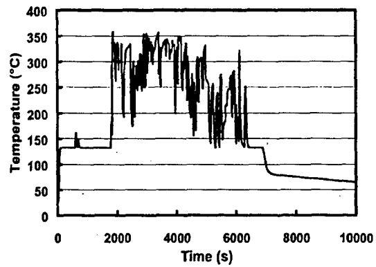
(b) Temperature-time mission history
