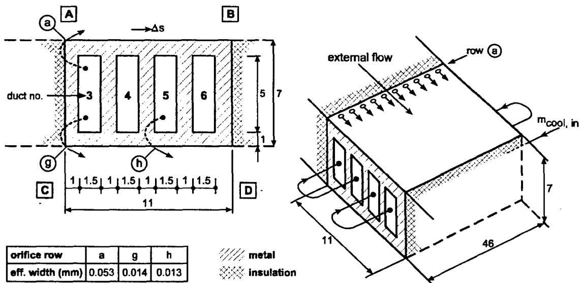
Figure 5: Model to approximate cooling gas temperature increase
