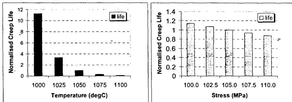
Figure 11: Temperature and stress sensitivity of creep life.
