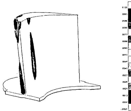
Figure 9: Creep damage distribution.
