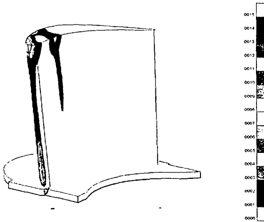
Figure 8: Fatigue damage distribution.
