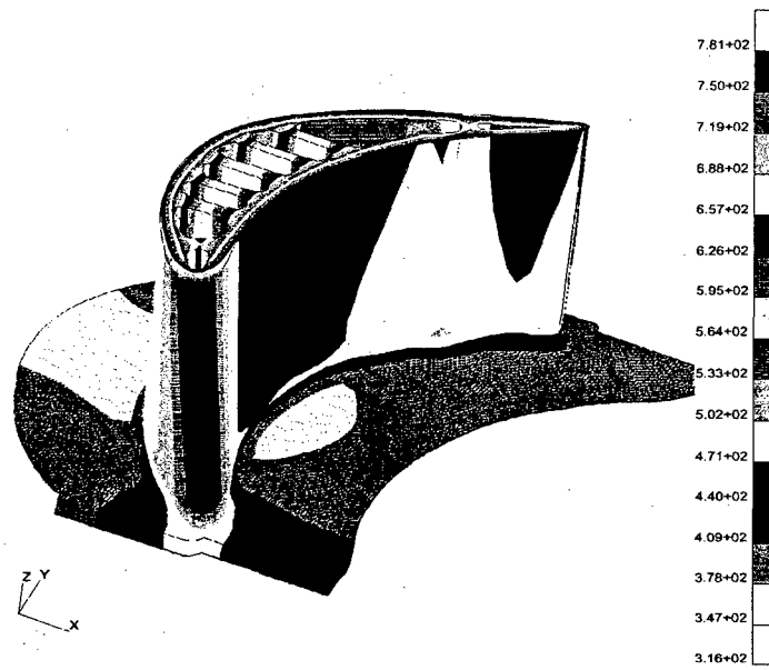
Figure 6: Temperature distribution ( ^{\circ}\text{C} ) in the lower half of an internally cooled turbine blade.
