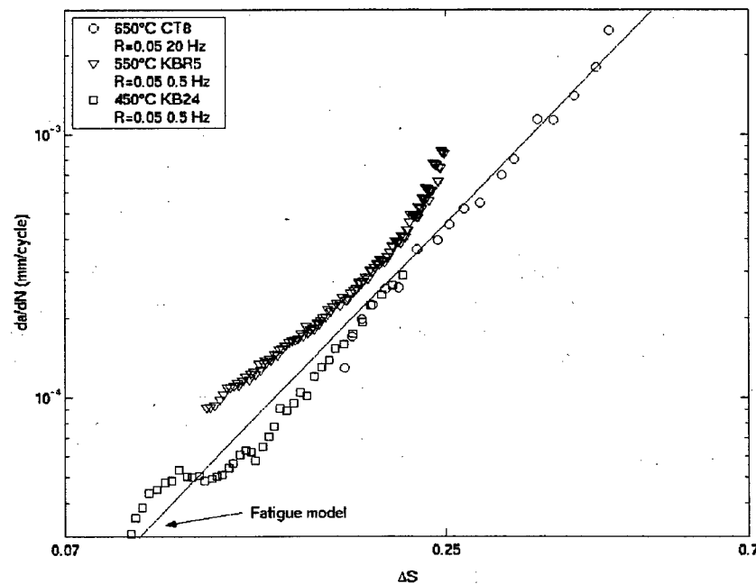
FIGURE 2. Identification of the pure fatigue model
