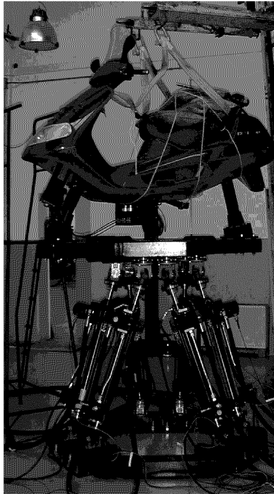
Figure 1 The MORIS motion simulator realized by PERCRO
