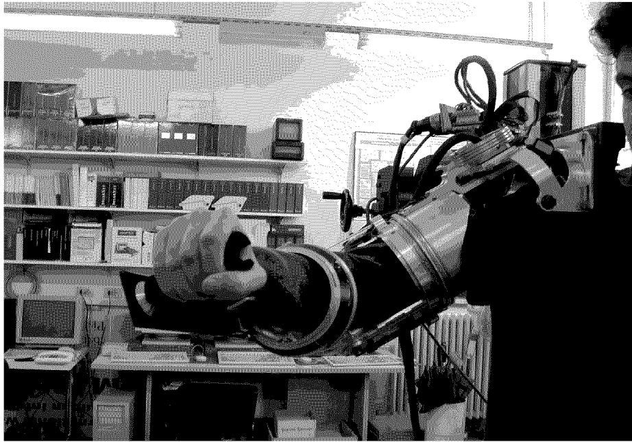
Figure 2 The arm force feedback exoskeleton
