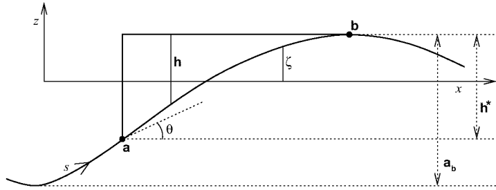
Figure 1: Geometry of the breaking wave.
