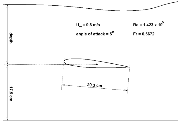
Figure 2: Experimental setup
