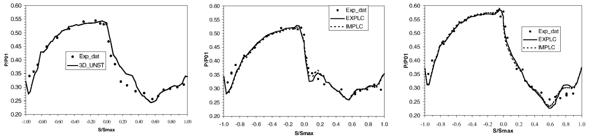
Figure 6: hub and tip time-averaged pressure profiles
