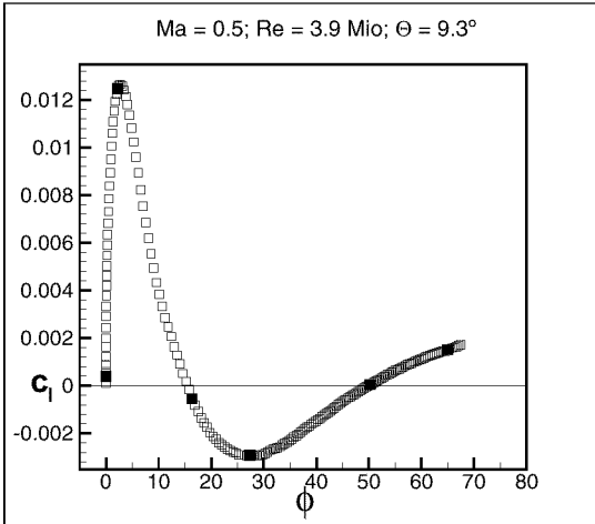
Figure 21: Roll-moment over roll angle, free-to-roll coupled simulation with flap
