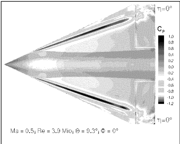
Figure 22: Surface pressure distribution, free-to-roll with flap motion
