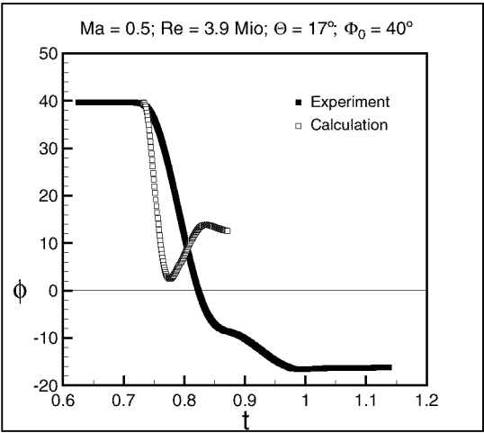
Figure 18: Roll angle \phi over time t , free-to-roll coupled simulation
