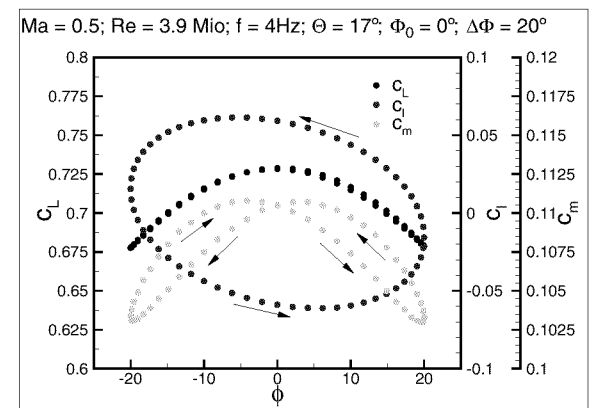
Figure 16: Integral lift, roll and pitching moment of oscillating delta wing flaps
