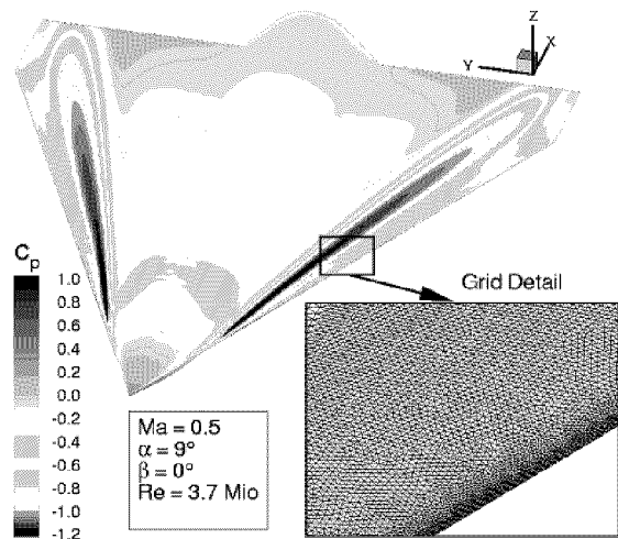
Figure 7: Tau-Code NS-Solution, adapted leading edge
