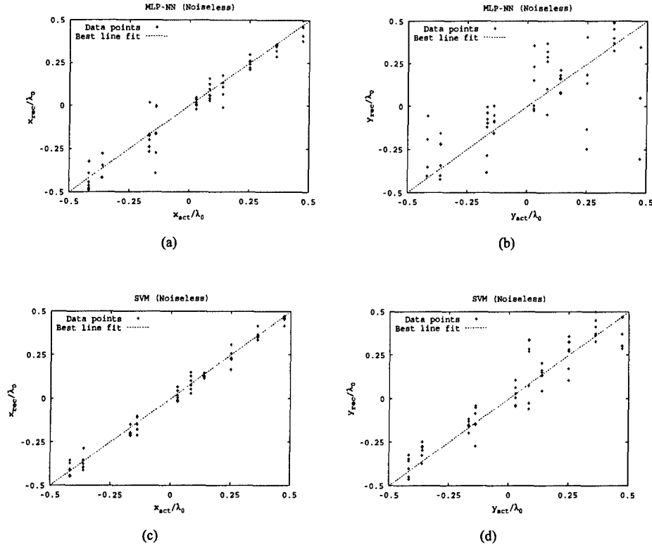
Fig. 4. Reconstructed data versus actual data (Noiseless Case). (a)-(b) MLP-NN approach, (c)-(d) SVM-based approach. (a)-(c) \frac{x_B}{\lambda_0} and (b)-(d) \frac{y_B}{\lambda_0}
